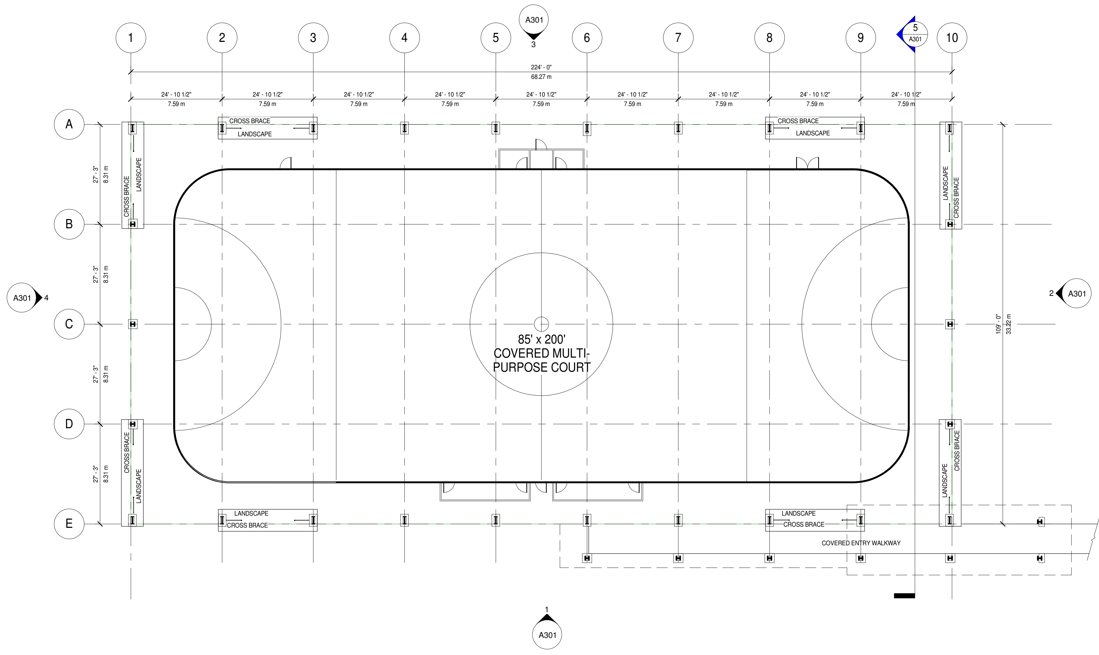
1 Level 1 1/16" = 1'-0"
